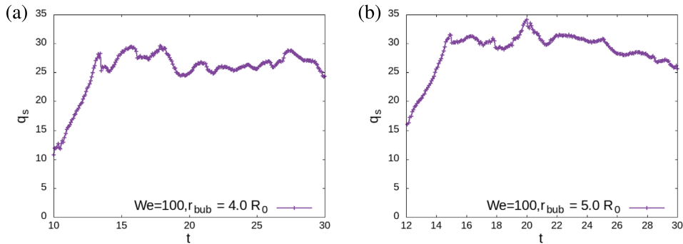
Figure 13. Swirl number q_s as a function of nondimensional time \bar{t} . Simulations at Re = 5000 , We = 100 with (a) r_B = 4 , (b) r_B = 5 .
