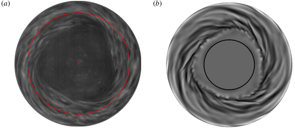
FIGURE 14. (Colour online) (a) Experiment at G = 0.1856 , Re = 30\,000 and Fr = 0.0335 : top view of the water layer seeded with Kalliroscope flakes. The red circle at r = 0.8 indicates the position of the line captured for the spatio-temporal diagram of figure 15(a). (b) Numerical simulation at G = 0.1856 , Re = 30\,000 and Fr = 0 : snapshot of the axial velocity at z = 0.84G . The periodic numerical domain (r, \theta) \in [0.4, 1] \times [0, (2/3)\pi] has been replicated along the azimuth; for r < 0.4 (inside the black circle) a zero axial velocity has been plotted.
