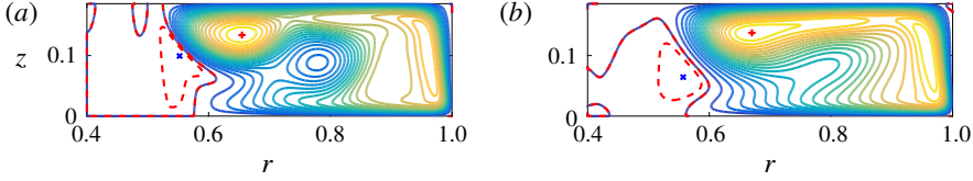
FIGURE 10. (Colour online) Streamlines of the meridional circulation for G = 0.1856 , Re = 30\,000 , computed from (a) \bar{V}_{2D} (respectively (b) \bar{V}_{3D} ). The graph consists of 21 equispaced solid contours of \psi between 0 and \psi_{max} = 2.1 \times 10^{-3} (respectively 1.98 \times 10^{-3} ) and one dashed contour at value (1/2)\psi_{min} with \psi_{min} = -1.12 \times 10^{-4} (respectively -0.924 \times 10^{-4} ). The locations of the points with maximum and minimum \psi are respectively indicated by the red and the blue cross.
