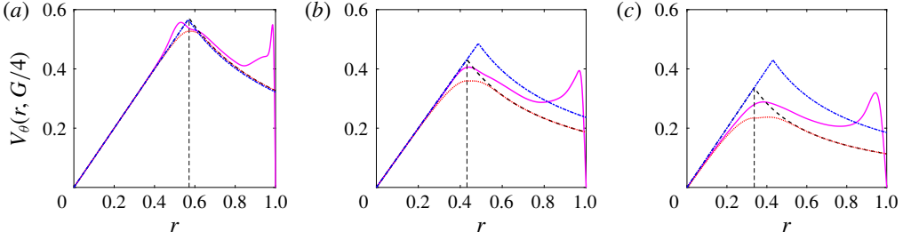
FIGURE 17. (Colour online) Comparison between azimuthal velocity profiles along the radius for aspect ratios (a) G = 0.1856 , (b) G = 0.5 and (c) G = 1 . Magenta solid: ROSE calculation at Re = 10\,000 and z = G/4 . Red dotted: distribution from Iga's (2017) model (the thin black dashed line shows the position of r_s^I as determined in this model respectively at 0.57, 0.43 and 0.34). Black dashed: ideal Rankine vortex model with core size r_s^I . Blue dash-dot: the TMBF model in Mougél (2014) with correction of the dissipation, leading to values r_s^{TMBF} = 0.57, 0.49 and 0.43 . Without corrections, this latter model would predict values 0.65, 0.58 and 0.52 respectively for the three aspect ratios.
