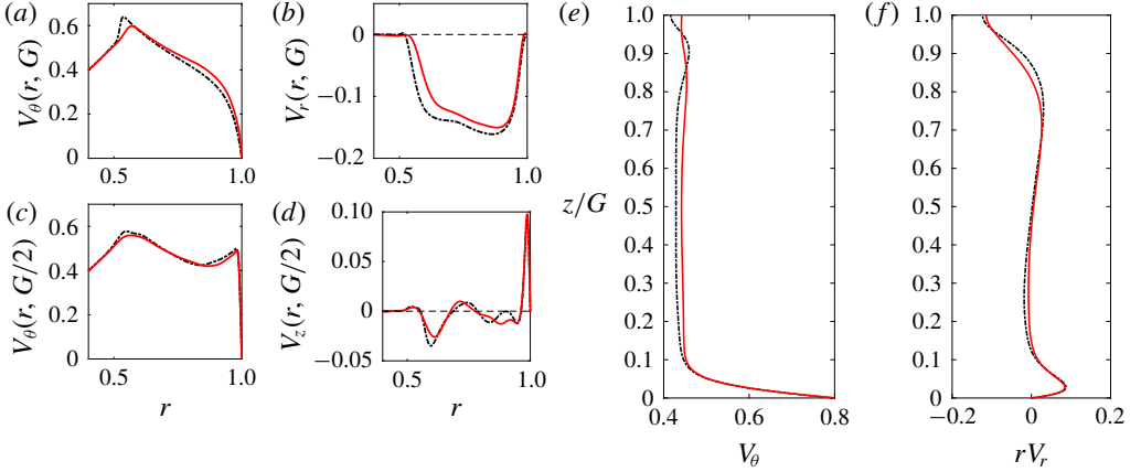
FIGURE 11. (Colour online) Profiles of mean velocities \bar{V}_{2D} (black dash-dotted lines) and \bar{V}_{3D} (red continuous lines) obtained by DNS for G=0.1856 , Re=30\,000 . Velocity profiles as in figure 4.
